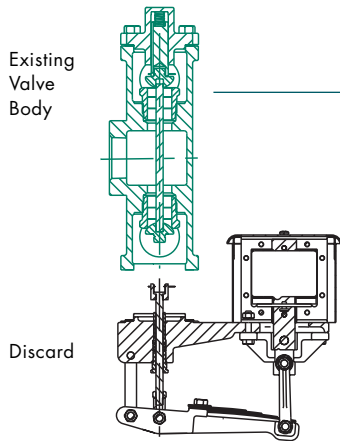
3-Way Solenoid Valve – Split
