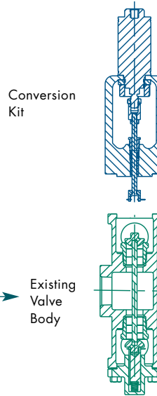
3-Way Cylinder Valve – Split
